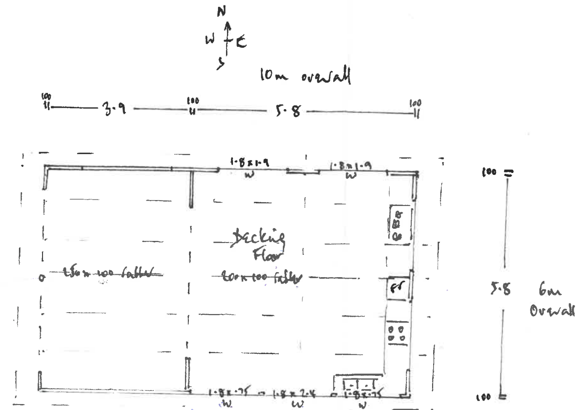
KITCHEN/DINING/LOUNGE Scale 1:100 6m x 10m 60m 2
